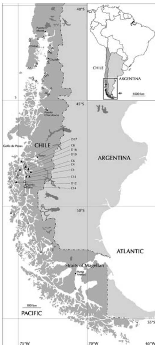
Fig. 1. Sampling sites in the Chilean fjord region. \Delta , sampled sites. \blacktriangle , sites where polyps were found. \circ , sites where medusae were found.
